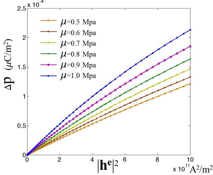
Figure 6: An elastic film in an electric and magnetic field.
