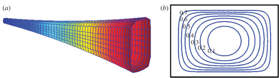
Figure 4. (a) The shape of the rods on the hairy sphere in figure 3d. (b) The cross section of the rod for a unit cell [0, 1.5] \times [0, 1] and various volume fractions. The number on each curve is the volume fraction of the inclusion. (Online version in colour.)
