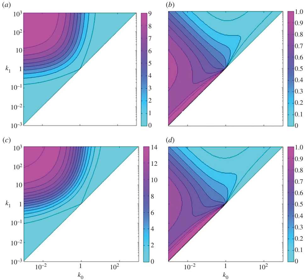
Figure 2. Contour plots of (a,c) the optimal amplification factor f = \tilde{f}^*(\sigma_0, \sigma_1, \rho, n) and (b,d) the optimal volume fraction \theta^* = \theta^*(\sigma_0, \sigma_1, \rho, n) . (a) f = \tilde{f}^*(\sigma_0, \sigma_1, \rho = 0.1, n = 2) ; (b) \theta^* = \theta^*(\sigma_0, \sigma_1, \rho = 0.1, n = 2) ; (c) f = \tilde{f}^*(\sigma_0, \sigma_1, \rho = 0.1, n = 3) and (d) \theta^* = \theta^*(\sigma_0, \sigma_1, \rho = 0.1, n = 3) . (Online version in colour.)
