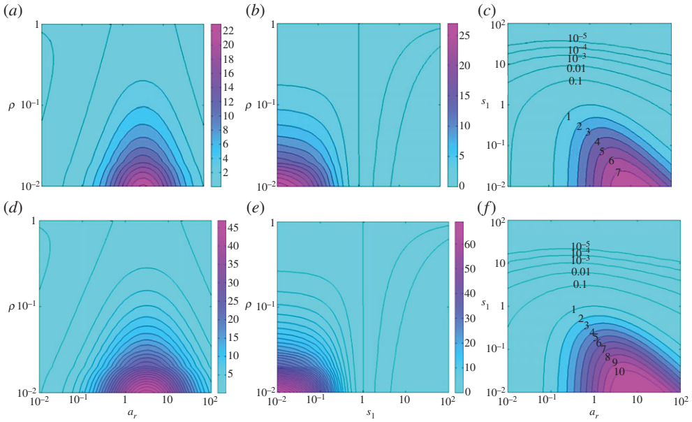
Figure 1. Contour plots of the amplification factor f = f(a_r, s_1, \rho, n) in two and three dimensions. (a) f = f(a_r, s_1 = 0.1, \rho, n = 2) ; (b) f = f(a_r = 1, s_1, \rho, n = 2) ; (c) f = f(a_r, s_1, \rho = 0.1, n = 2) ; (d) f = f(a_r, s_1 = 0.1, \rho, n = 3) ; (e) f = f(a_r = 1, s_1, \rho, n = 3) and (f) f = f(a_r, s_1, \rho = 0.1, n = 3) . (Online version in colour.)
