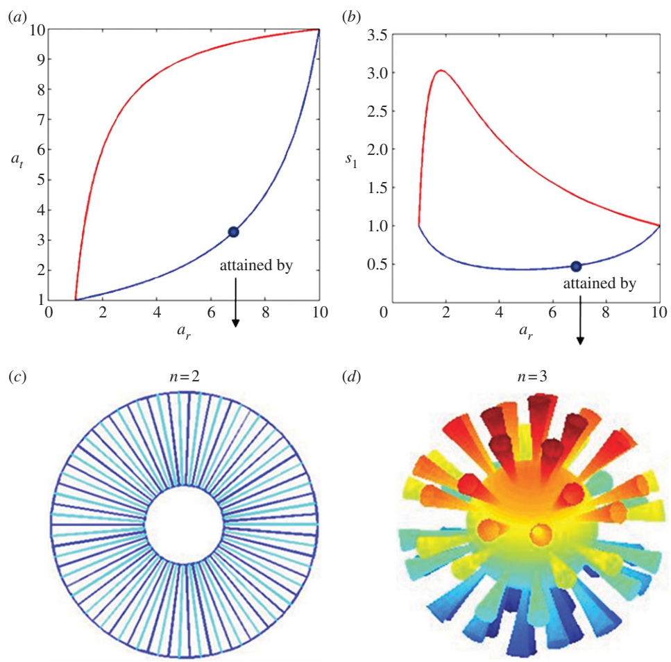
Figure 3. (a) The set \mathcal{C} to which the pair (a_r, a_t) necessarily belong to; (b) the set of (a_r, s_1 = a_t/a_r) if (a_r, a_t) \in \mathcal{C} ; (c) a two-dimensional microstructure of the composite of \sigma_0 \mathbf{I}, \sigma_1 \mathbf{I} (spike wheel) such that the effective tensor of the composite has the form (3.2) and the pair (a_r, a_t) attain a point on the lower boundary of the set \mathcal{C} and (d) a three-dimensional microstructure (hairy sphere) of the composite of \sigma_0 \mathbf{I}, \sigma_1 \mathbf{I} such that the effective tensor of the composite has the form (3.2) and the pair (a_r, a_t) attain a point on the lower boundary of the set \mathcal{C} . The tapered rod (hair) on the sphere and its cross section are shown in figure 4a,b. (Online version in colour.)
