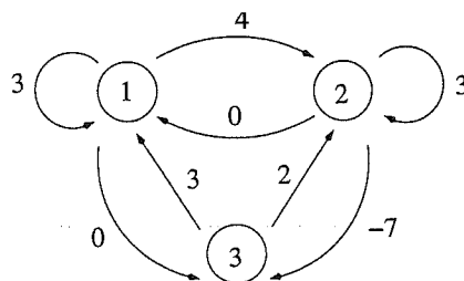
FIGURE 1. An additive version of Richman games
