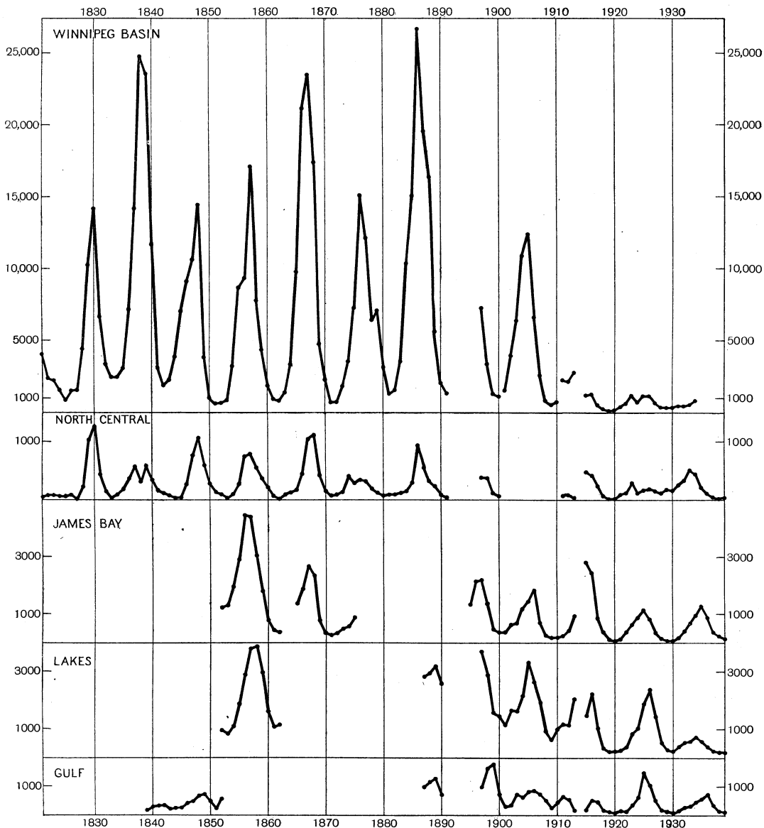
Fig. 9. Lynx fur returns of the Hudson's Bay Company, grouped into regions (Winnipeg Basin, North Central, James Bay, Lakes, Gulf).
